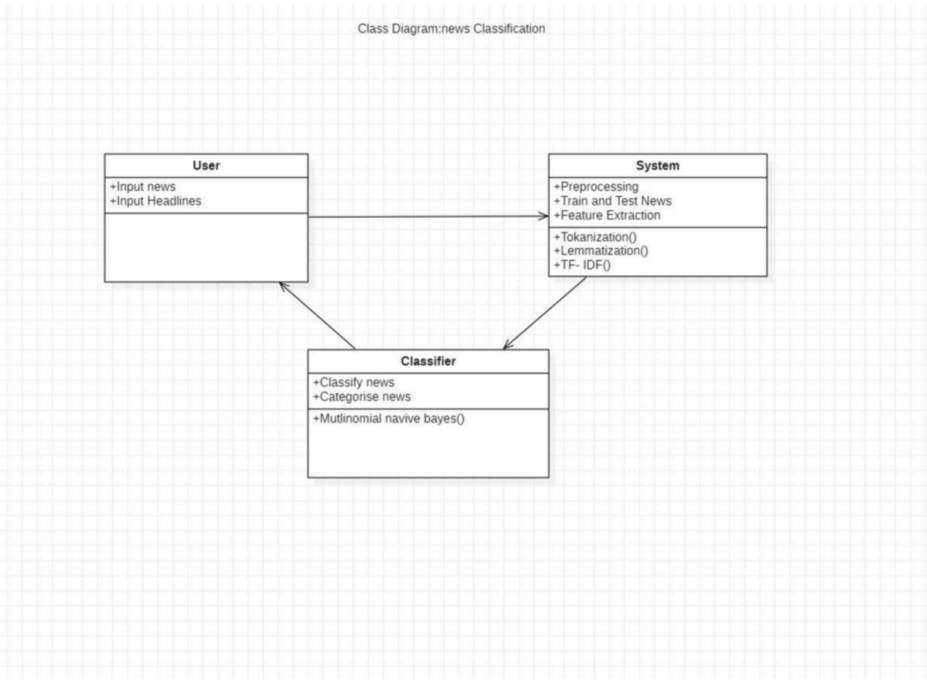
FIGURE 2: Class Diagram
