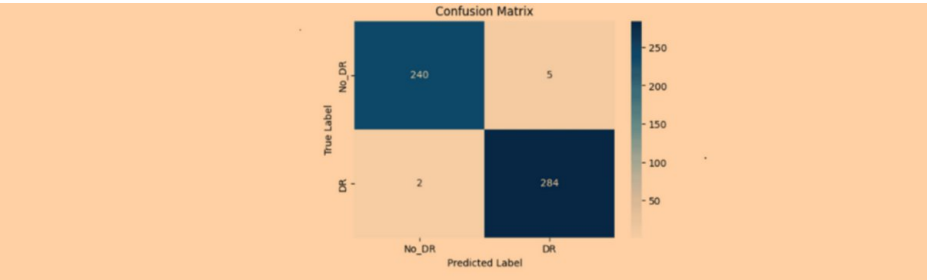
FIGURE 3: Confusion matrix
