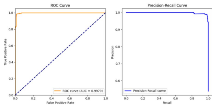
FIGURE 4: ROC and Precision-Recall curves
