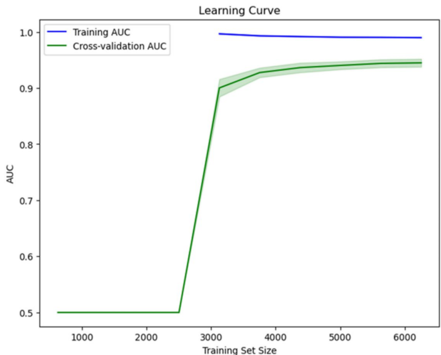
FIGURE 13: Learning curve
