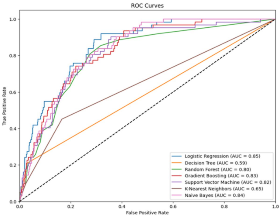
FIGURE 3: ROC curve for baseline algorithms
