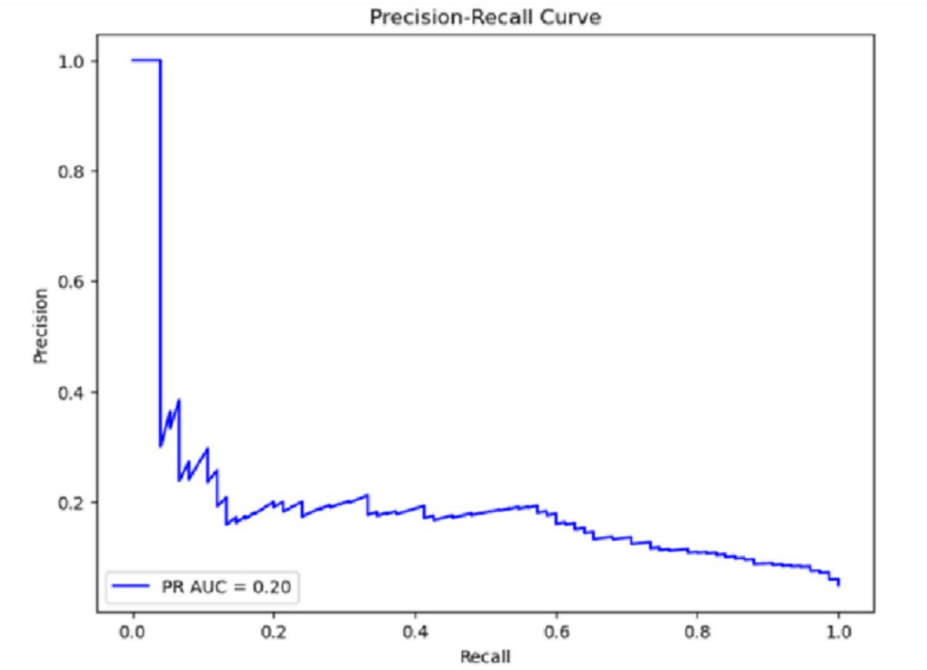
FIGURE 11: Precision-recall curve
