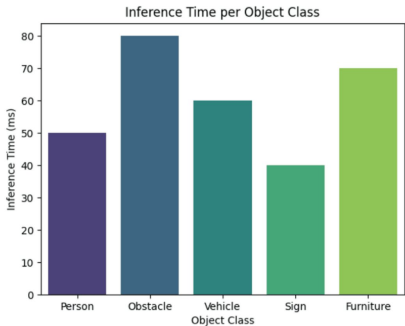
FIGURE 5: Inference time per object class
