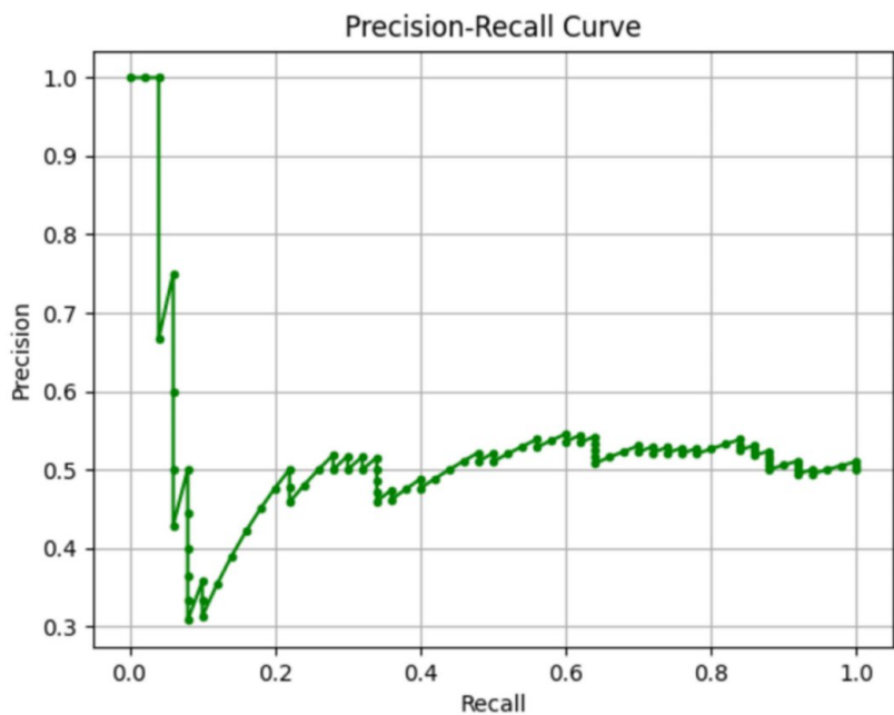
FIGURE 4: Precision-recall curve
