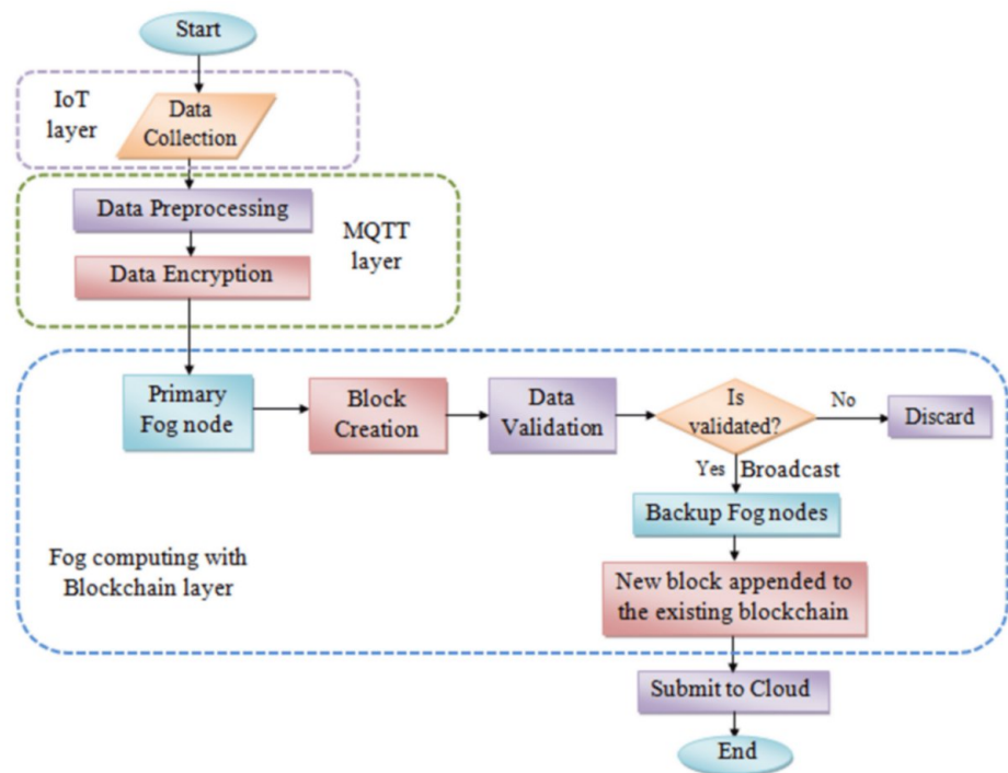
FIGURE 4: Data flow diagram of the proposed system
