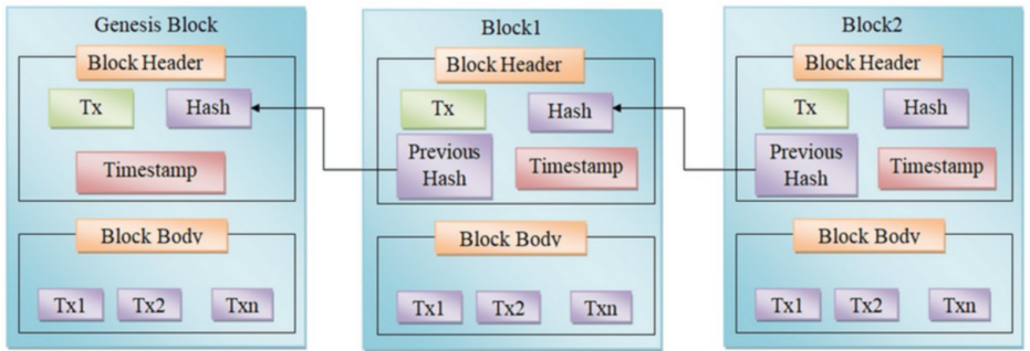
FIGURE 2: Blockchain
