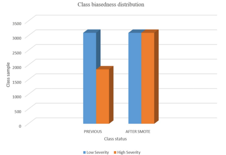
FIGURE 6: Distribution of ground truth before and after synthetic minority oversampling
