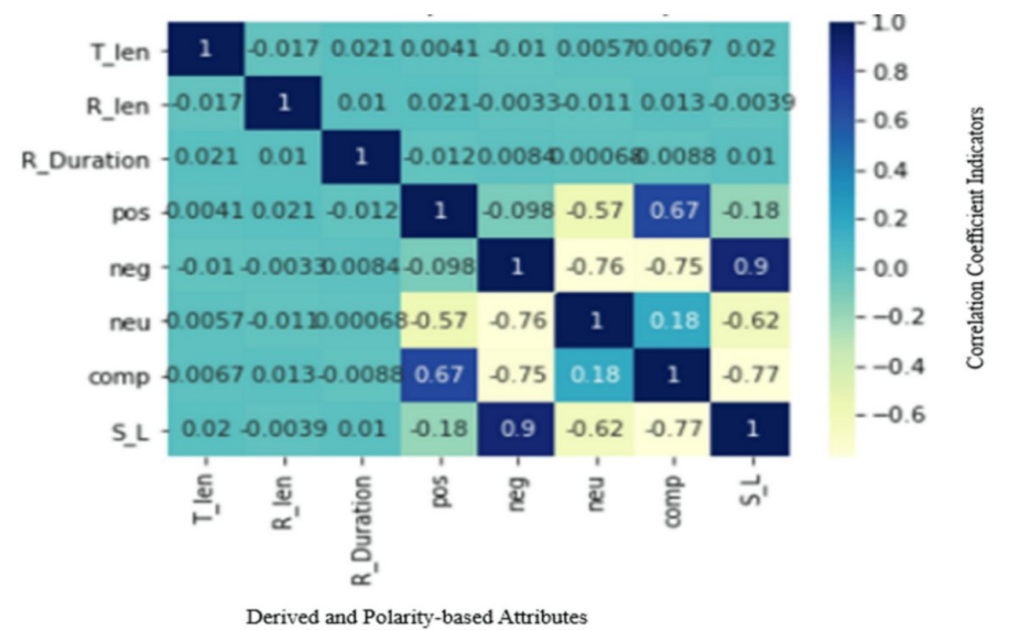
FIGURE 4: Correlation coefficient plot of the predictive attributes for multicollinearity test
