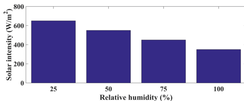
FIGURE 7: Comparison between solar intensity and relative humidity
