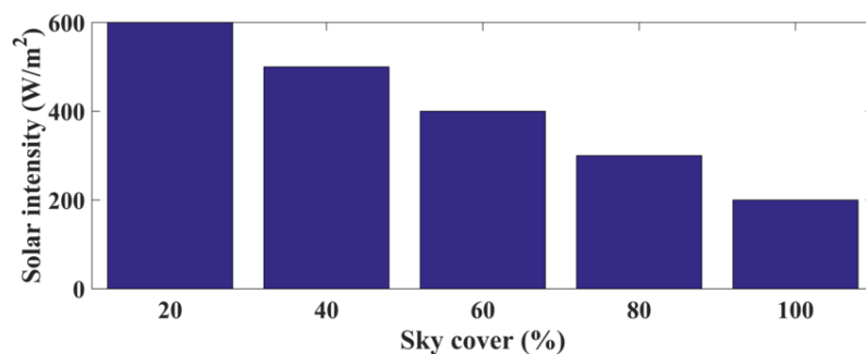
FIGURE 6: Comparison between solar intensity and sky cover
