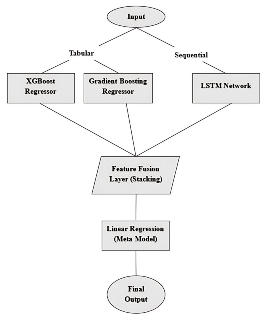
FIGURE 1: Architecture of EStack Fusion LSTM, Long Short-Term Memory
