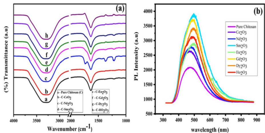
FIGURE 2: (a) FTIR spectra of pure chitosan and Ch-LO and (b) photoluminance of pure chitosan and Ch-LO
