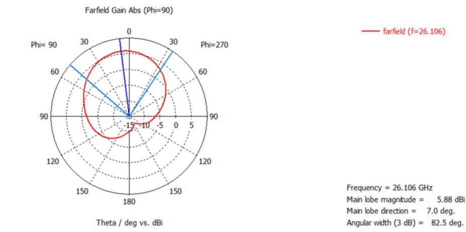
FIGURE 10: 2D radiation pattern of DGS-loaded half-moon-shaped patch antenna at \phi=90^\circ
