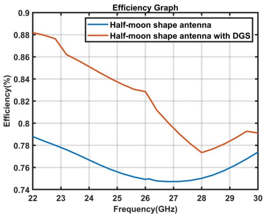
FIGURE 5: Comparative efficiency between half-moon-shaped antenna and DGS-loaded antenna
