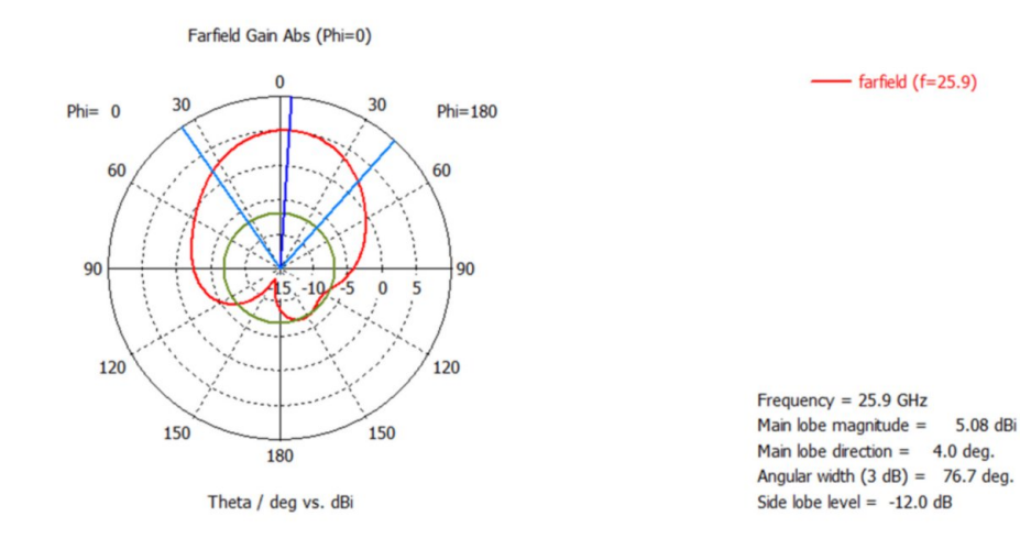
FIGURE 7: 2D radiation pattern of half-moon-shaped patch antenna at \phi=0^\circ
