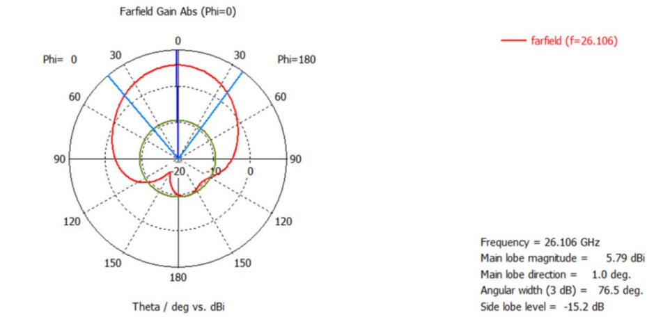
FIGURE 9: 2D radiation pattern of DGS-loaded half-moon-shaped patch antenna at \varphi= 0^\circ
