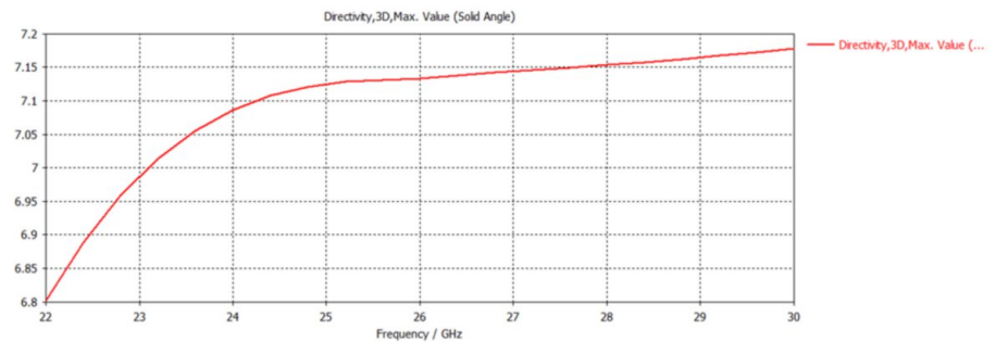
FIGURE 6: Directivity of DGS-loaded half-moon-shaped antenna DGS, Defected Ground Structure
