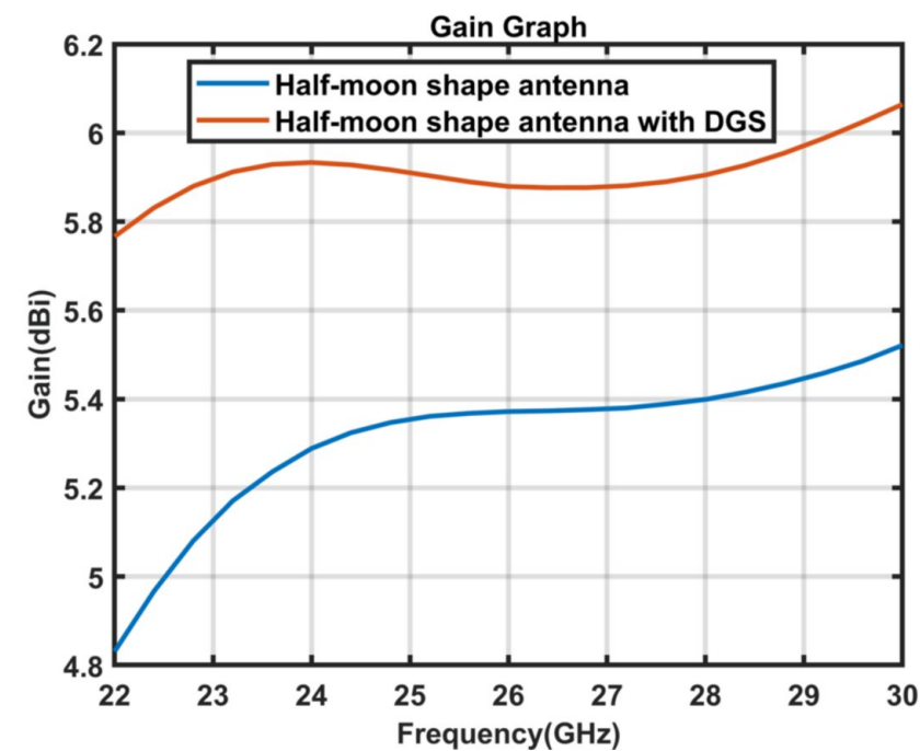
FIGURE 4: Comparative gain between half-moon-shaped antenna and DGS-loaded antenna
