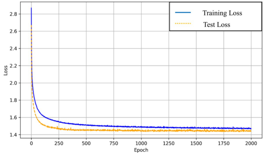
FIGURE 7: Loss plot for the best fold.
