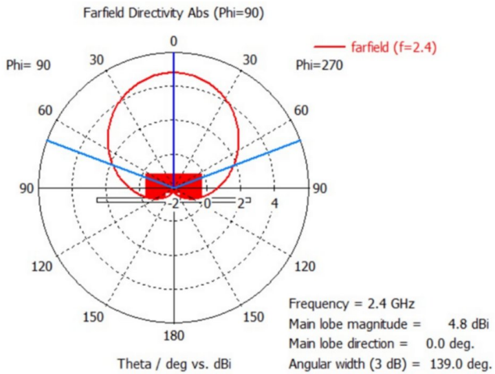
FIGURE 11: Far-field 2D directivity of the proposed antenna unit
