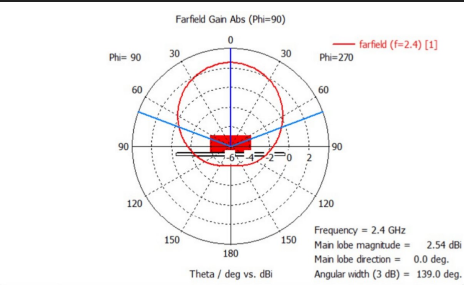
FIGURE 9: Far-field 2D gain of the proposed antenna unit
