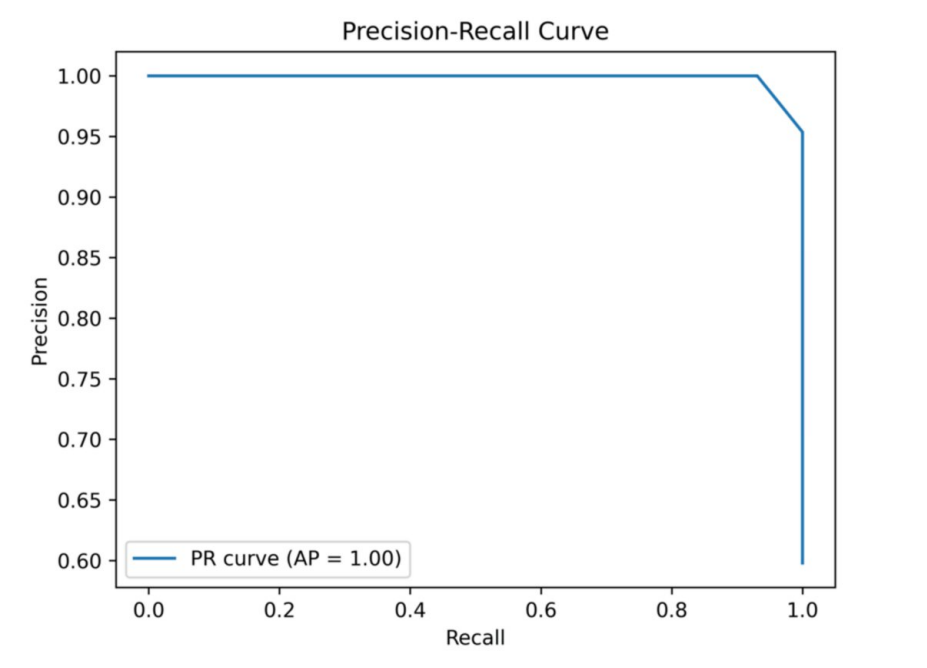
FIGURE 6: Precision-Recall Curve of the Proposed Model AP, Average Precision; PR, Precision-Recall
