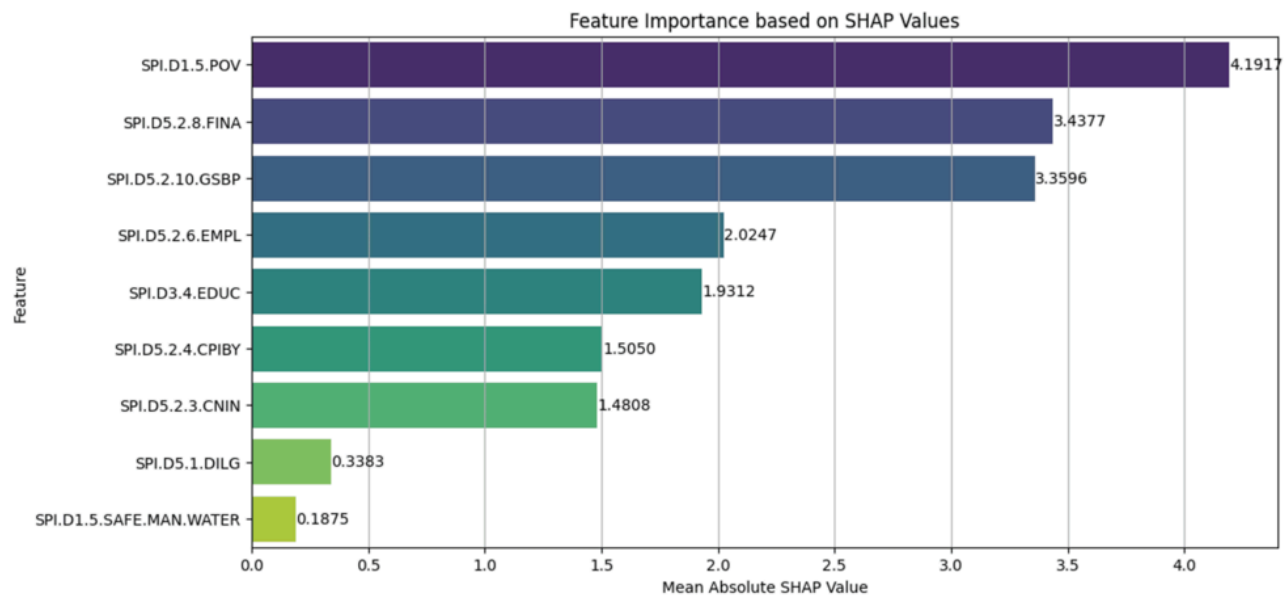
FIGURE 10: Feature importance analysis based on SHAP values, demonstrating the contribution of each feature to the model's predictions. Higher mean absolute SHAP values indicate a stronger impact on the model's output, with SPI.D1.5.POV being the most influential feature.
