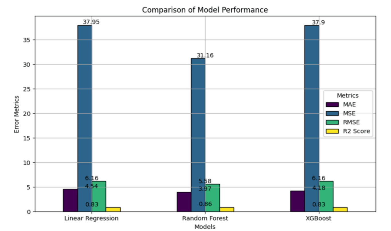
FIGURE 9: Performance assessment of Linear Regression, Random Forest, and XGBoost models using evaluation metrics: Mean Absolute Error (MAE), Mean Squared Error (MSE), Root Mean Squared Error (RMSE) and R^2 Score. Lower MAE, MSE, and RMSE values specify better predictive accuracy, while a higher R^2 Score reflects a stronger model fit.
