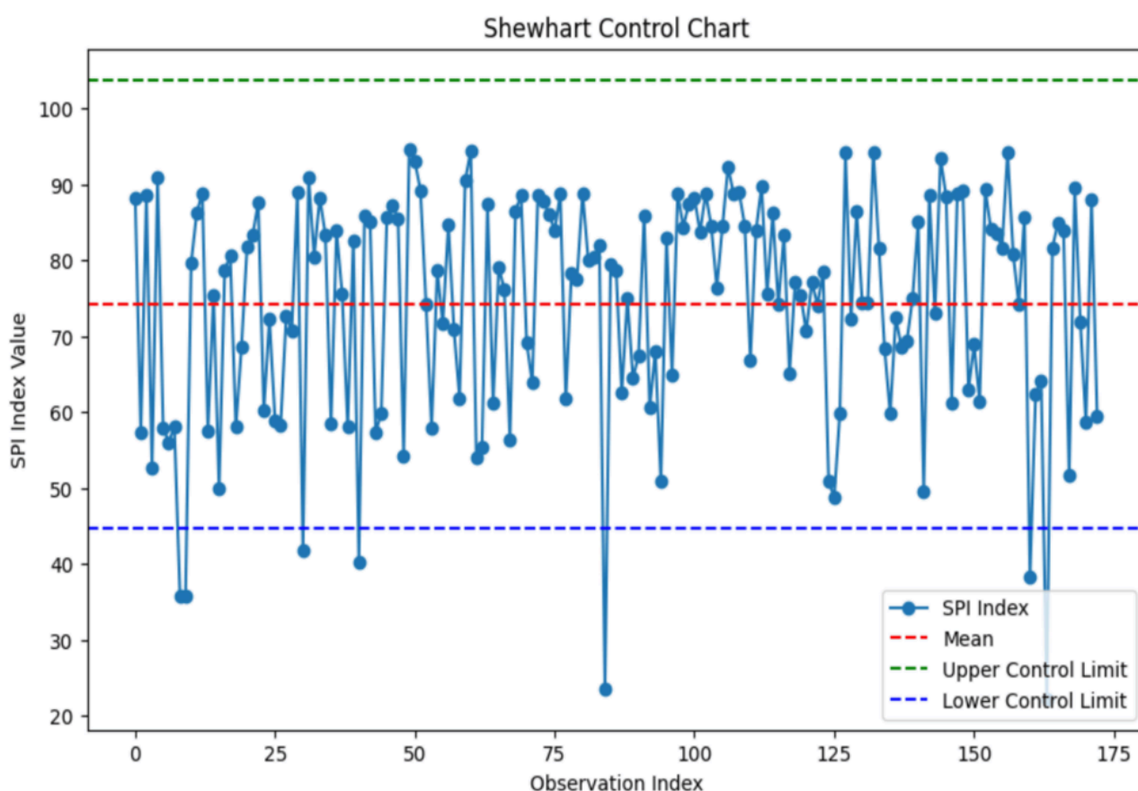
FIGURE 13: SPI index values using Shewhart Control charts that validate process variation with mean (red), upper control limit (green), and lower control limit (blue).
