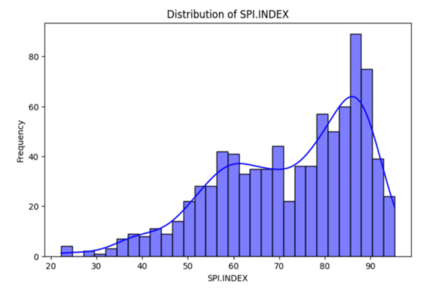
FIGURE 6: Distribution of SPI.INDEX – The histogram demonstrates the frequency distribution of SPI.INDEX values covered with a density curve to show the overall pattern and variability in the data.
