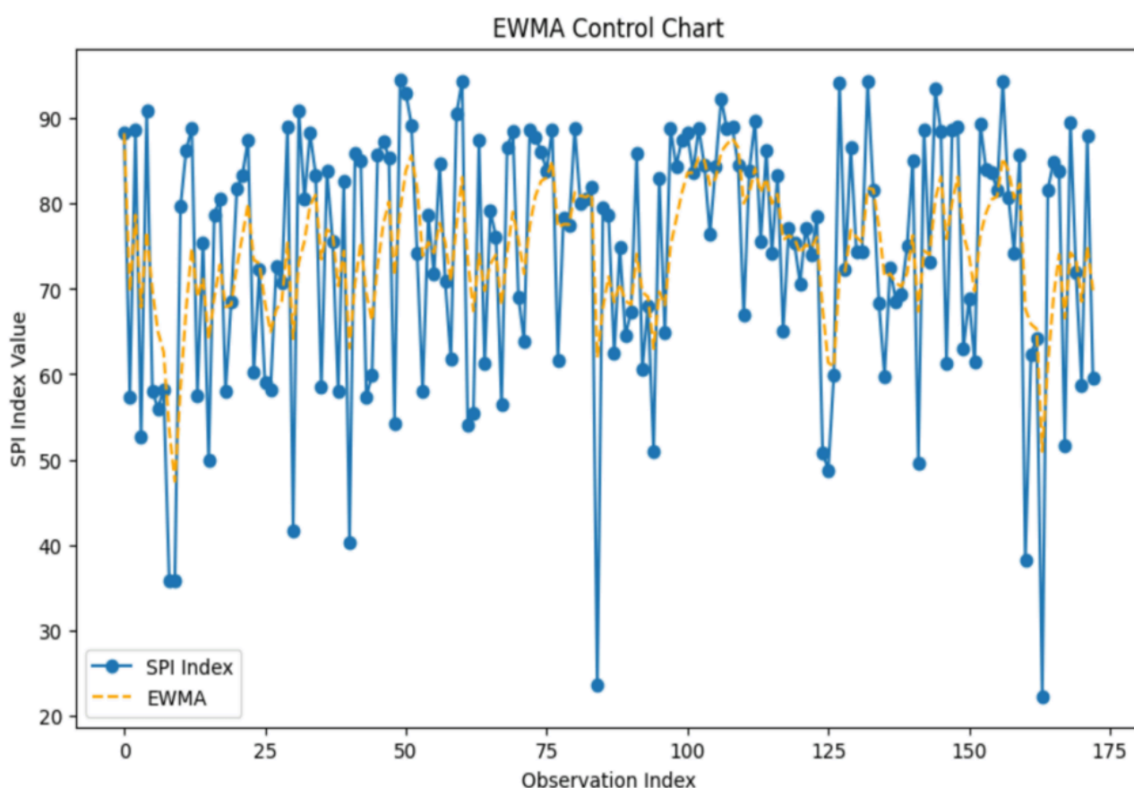
FIGURE 14: SPI index values using Exponentially Weighted Moving Average (EWMA) control chart showing smoothed trend (dashed yellow) alongside raw observations (blue).
