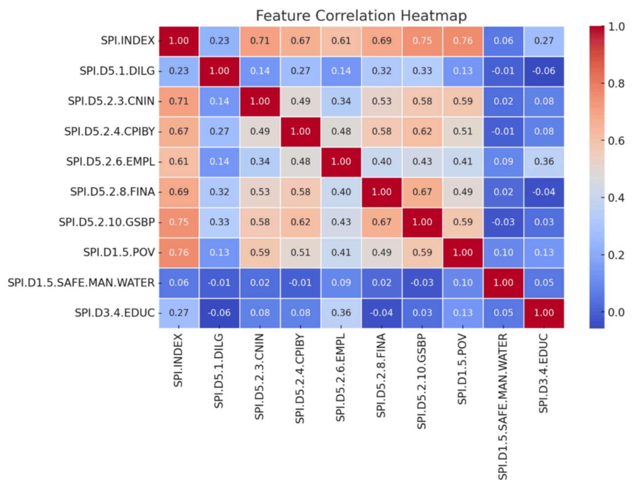
FIGURE 7: Feature Correlation Heatmap – The heatmap visualizes the correlation coefficients between SPI.INDEX and various financial and socioeconomic indicators, highlighting the strength and direction of relationships among the variables.
