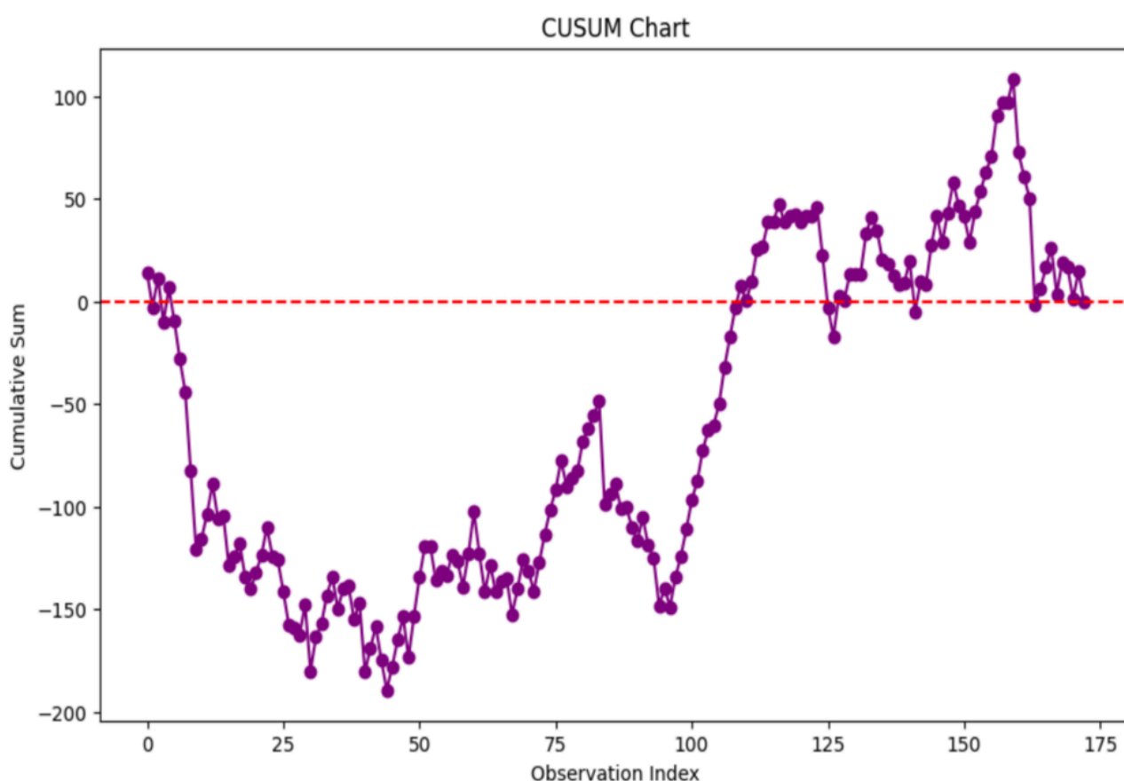
FIGURE 15: Cumulative Sum (CUSUM) control chart illustrating the cumulative deviation of SPI index values from the target mean, highlighting potential shifts in the process over time.
