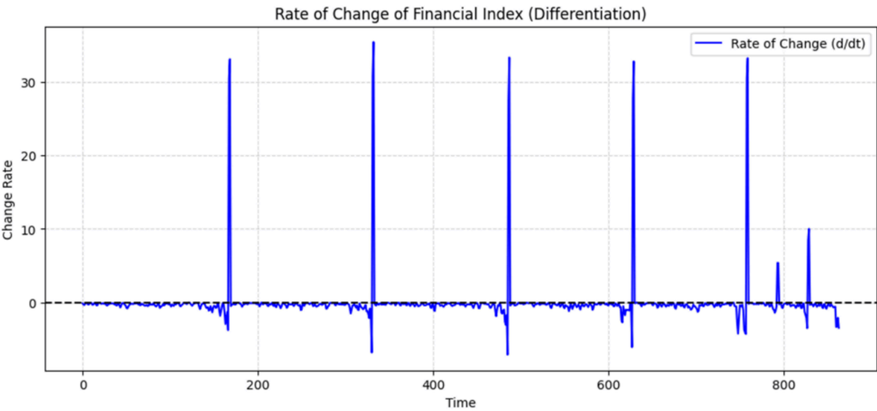
FIGURE 16: Rate of change of the financial index over time, highlighting fluctuations and potential anomalies using differentiation.
