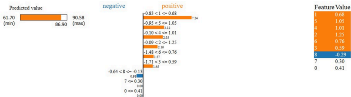
FIGURE 17: SHAP plot illustrates the contribution of different feature value ranges to the model's predicted output. Positive contributions are shown in orange, while negative contributions are in blue, with the predicted value represented on the left.
