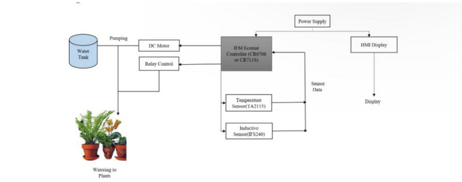
FIGURE 1: Block Diagram
