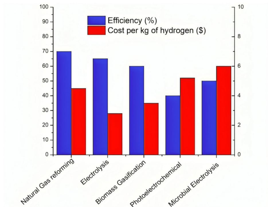
FIGURE 4: Hydrogen production methods and efficiency
